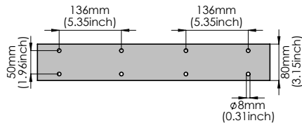
BOTTOM VIEW 20" (508mm)
