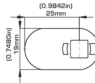
Cam - 25mm offset
