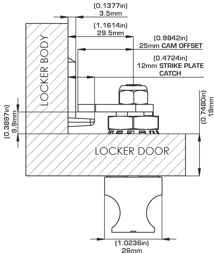
Top View
